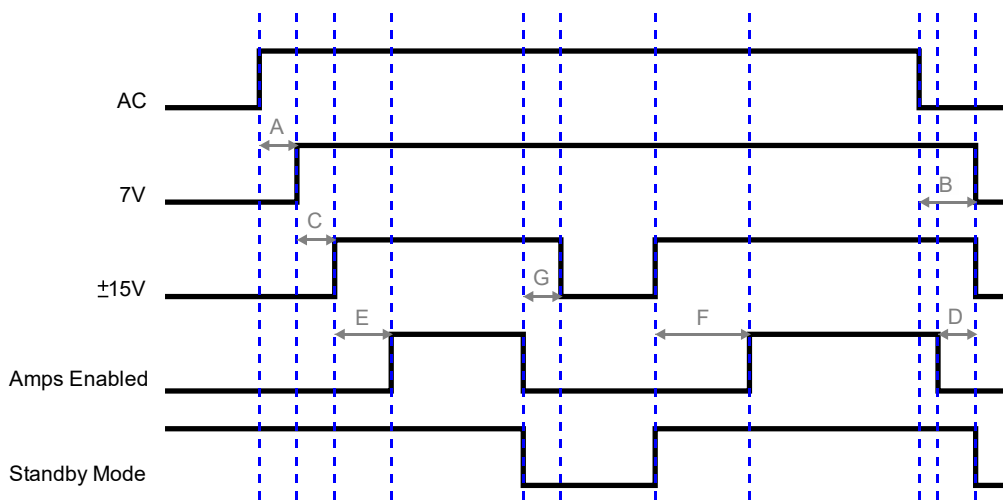
Figure 4-6: Power up/down timing diagram
