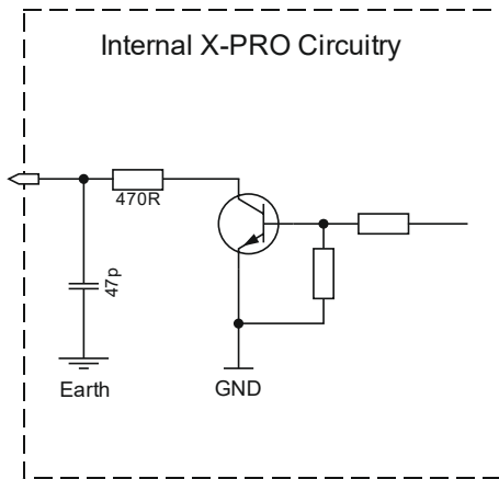
Figure 4-3: Open Collector output
