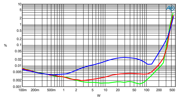
THD+N vs. Po, Channel 2 & 3, 100Hz (green), 1kHz (red), 6,67kHz (blue), 8Ω
