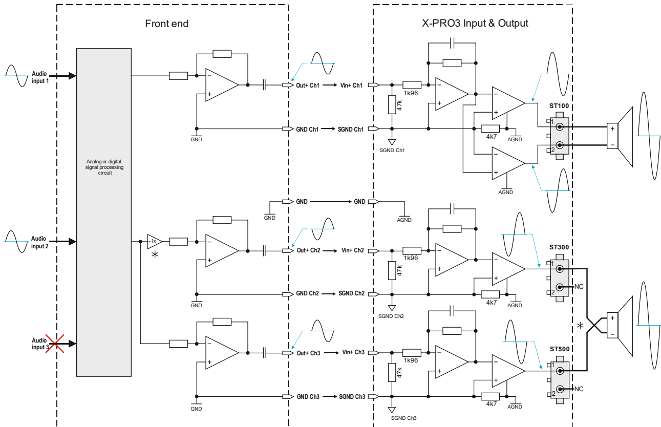
Figure 5-2: X-PRO in BTL configuration
