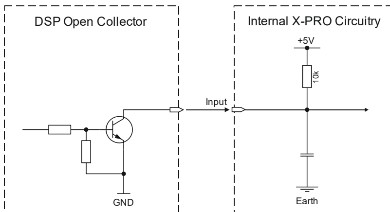
Figure 4-4: Input for Open Collector control
