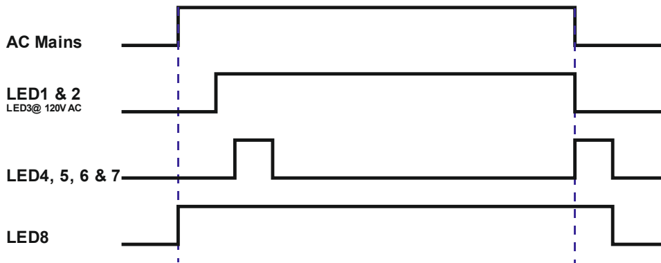
Figure 4-2: LED timing during start-up and shut-down
