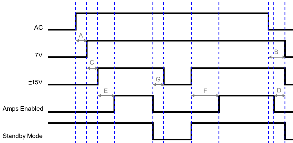
Figure 4-6: Power Up/Down timing diagram
