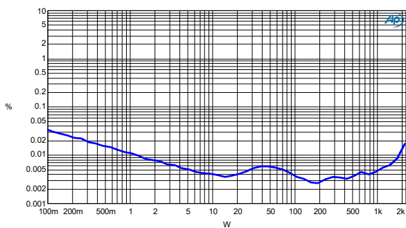
TIM vs. power, R_L=4 Ohm channel 1
