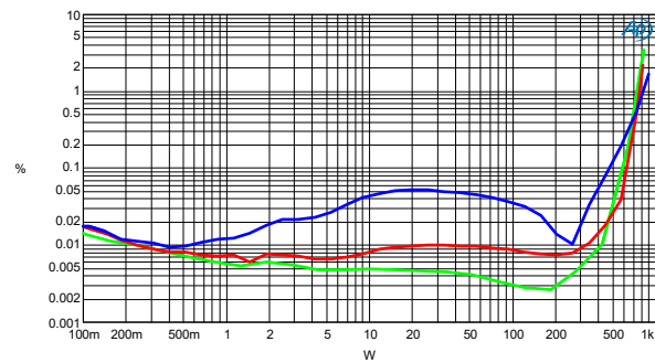
THD+N vs. Po, Channel 2 & 3, 100Hz (green), 1kHz (red), 6,67kHz (blue), 4Ω
