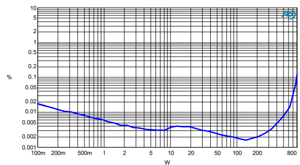
TIM vs. power, R_L=4 Ohm channel 2/3
