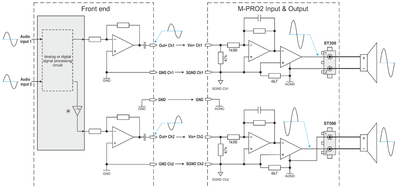
Figure 5-1: Single Ended mode, input & configuration
