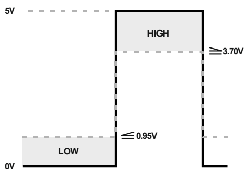
Figure 4-5: High and Low voltage levels for logic input.
