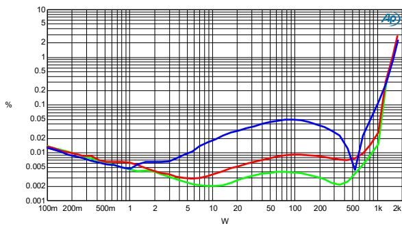
THD+N vs. Po, Channel 1, 100Hz (green), 1kHz (red), 6,67kHz (blue), 8Ω
