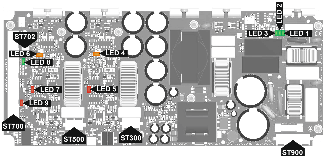
Figure 4-1: M-PRO2 connections and LED indicators
