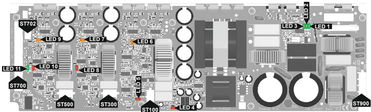
Figure 4-1: X-PRO3 connectors and LEDs
