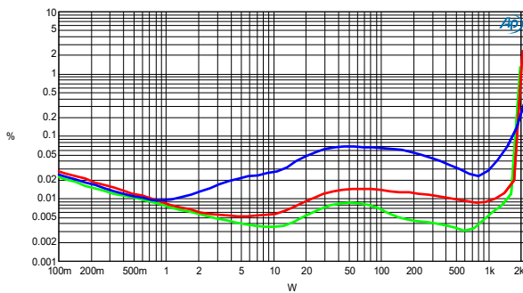
THD+N vs. Po, Channel 1, 100Hz (green), 1kHz (red), 6,67kHz (blue), 4Ω 1
