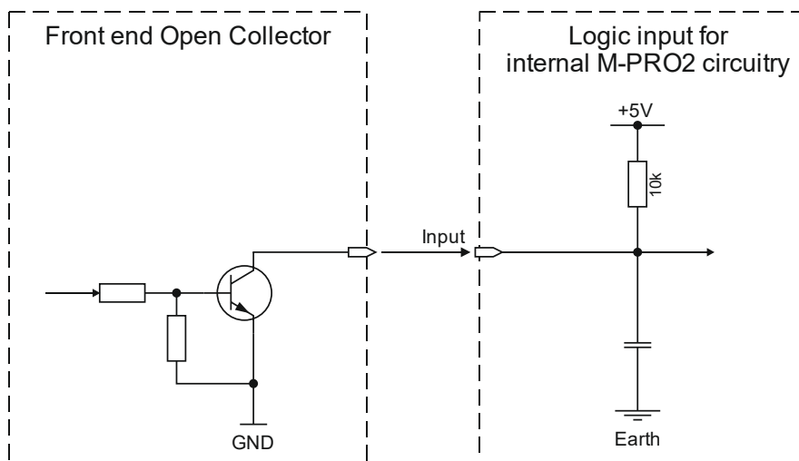
Figure 4-4: Open Collector Output from front-end used as Input for M-PRO2
