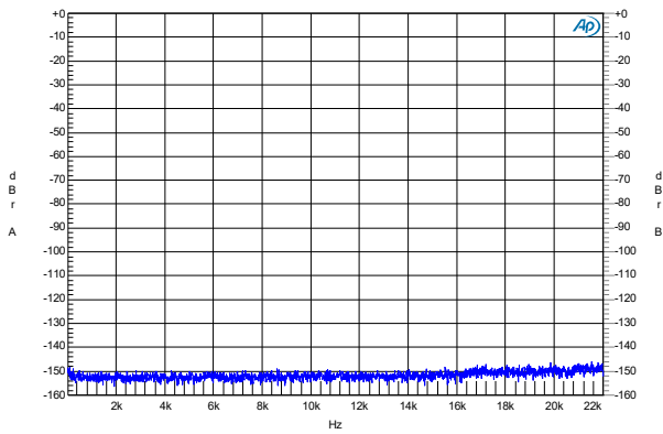
FFT, Channel 1, 4 Ohm, Idle
