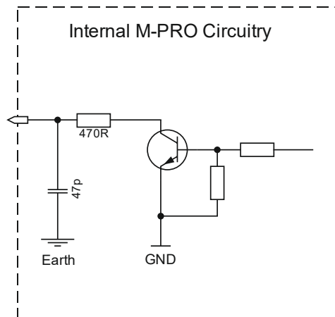
Figure 4-3: Open Collector Output from M-PRO2 module
