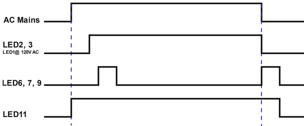
Figure 4-2: LED timing during start-up and shut-down
