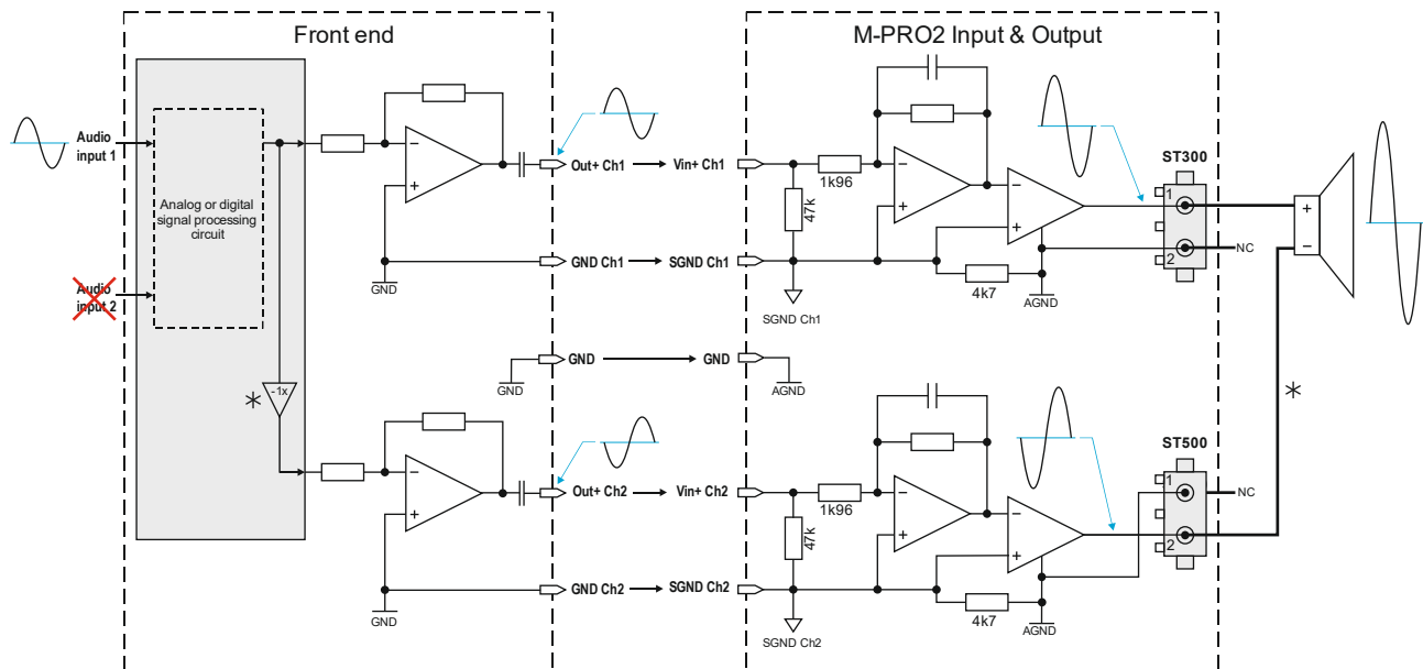
Figure 5-2: Bridge Tied Load mode, input & output configuration
