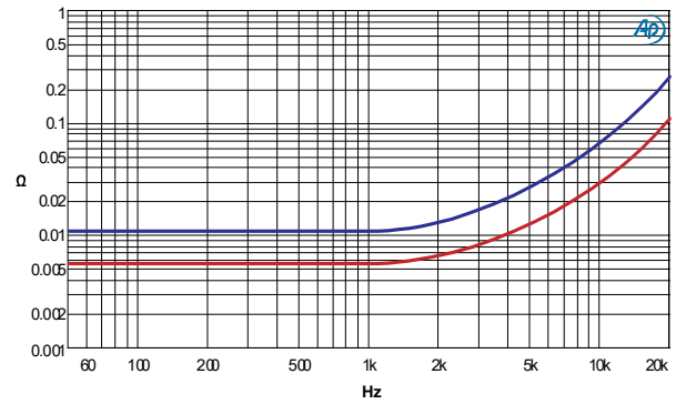
Output impedance, Channel 2/3, I_{out}=1A_{RMS} , Channel 1, I_{out}=1A_{RMS}
