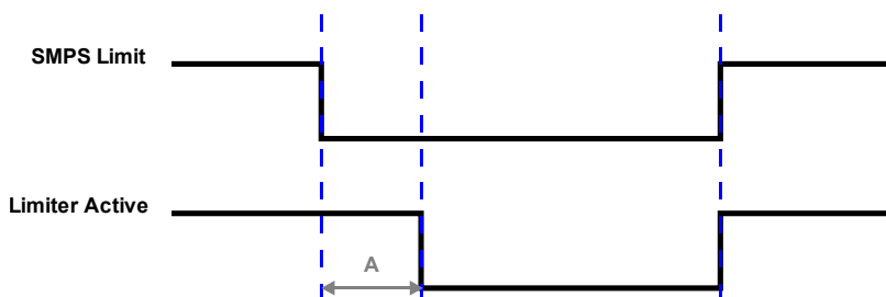
Figure 7-1: SMPS limit, A = Typically 1 sec.
