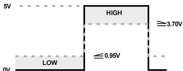
Figure 4-5: High and Low voltage levels for logic input
