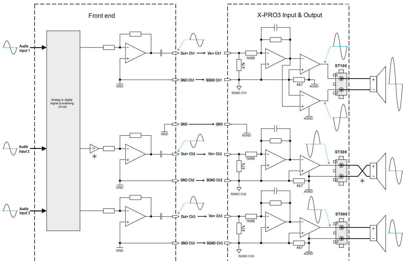
Figure 5-1: X-PRO in SE configuration
