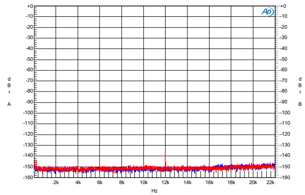
FFT, Channel 1 (Blue) & 2 (Red), 4 Ohm, Idle
